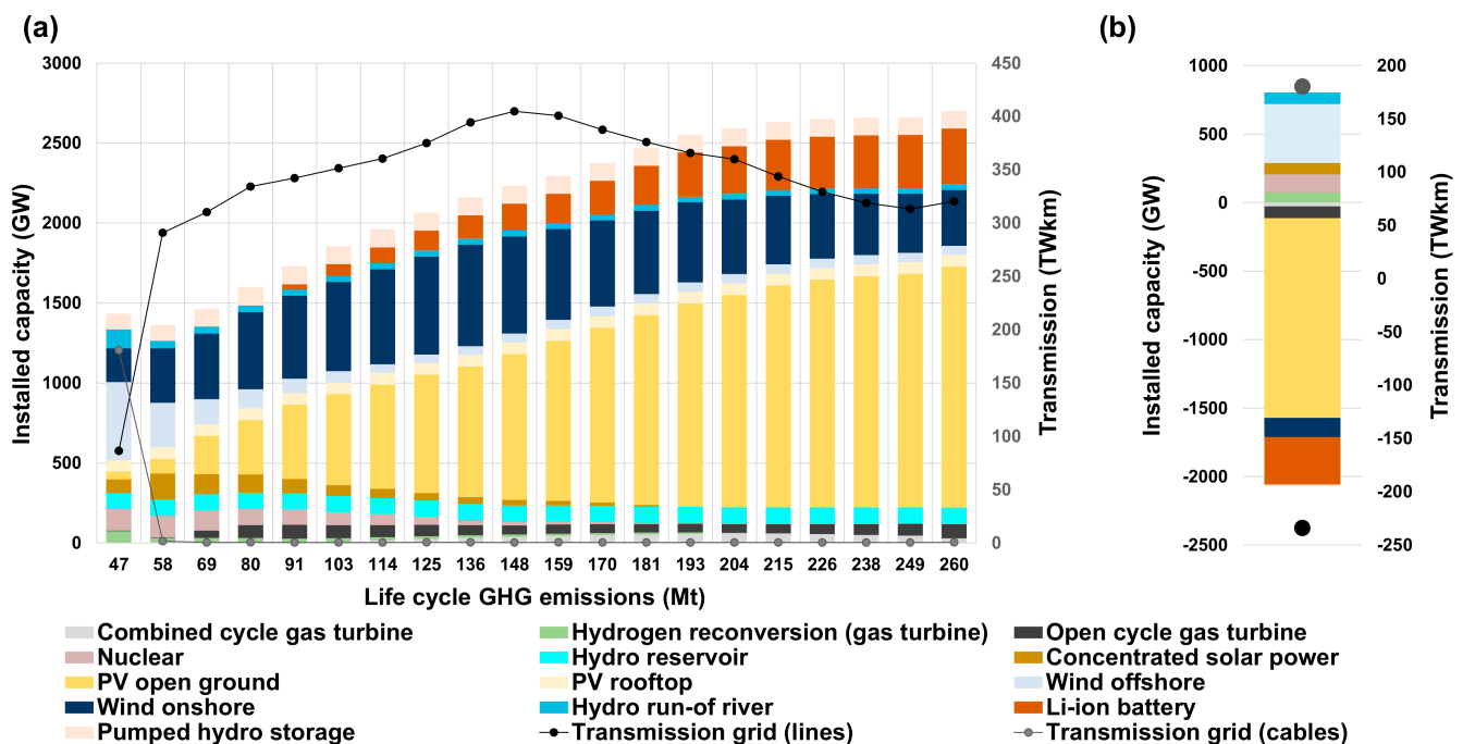
Figure 4. Power plant and power storage portfolio and transmission capacities in the EUNA region. Panel (a) shows the power plant and storage portfolio (left y-axis) and the grid installations (right y-axis) for each solution on the pareto front (Figure 3). Panel (b) shows the technology specific differences between the cost-optimal solution and the least life cycle GHG emissions-intensive solution for both, power generation and storage capacities and grid. Technologies with less than a 1% share of capacity in any solution are not shown for the sake of clarity.
